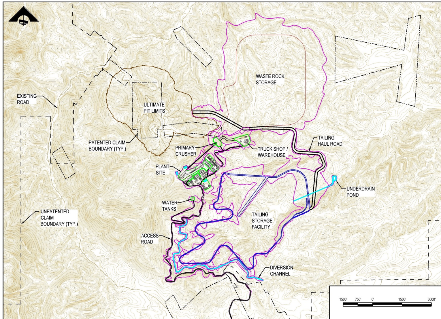
Figure 1-2: Mine Site Plan (000-GA-001)
